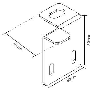
Lower auxiliary bracket
