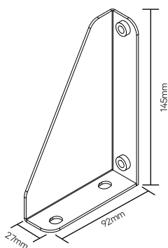
Upper bracket
